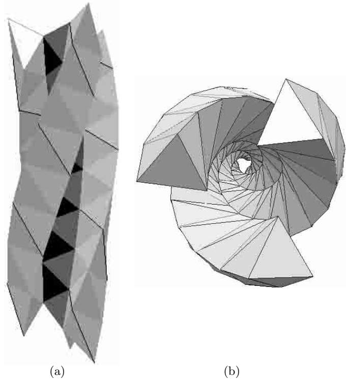
Fig. 14. Illustration of the collagen model of Sadoc and Rivier, produced by our projection method. Three columns of packed tetrahedra twist around a central B-C helix. The type \{2\} helices marked in black correspond to the peptide chains. (a) General view of the four B-C helices. (b) Perspective view along the axis.
