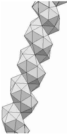
Fig. 11. A helix of interpenetrating icosahedra.
