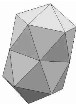
Fig. 1. The “double icosahedron” cluster.
