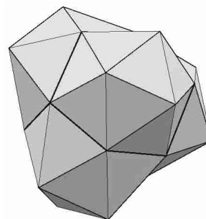
Fig. 3. Four interpenetrating icosahedra, sharing a central tetrahedron.
