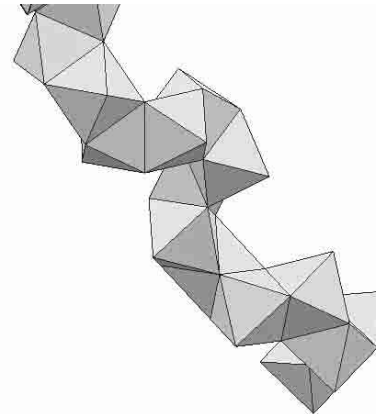
Fig. 9. A helix of octahedra.
