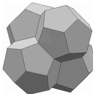
Fig. 4. Four pentagonal dodecahedra in face contact.
