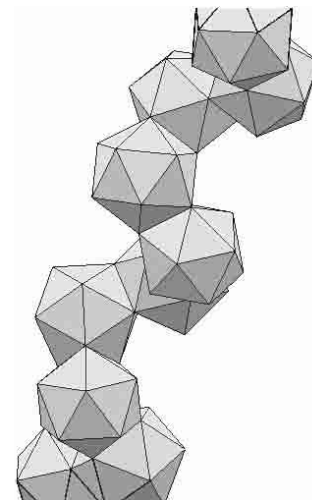
Fig. 10. A helix of icosahedra in face contact.
